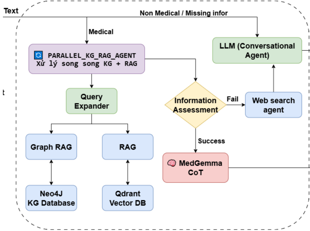
Figure 3.3: Text Module architecture for medical knowledge retrieval
