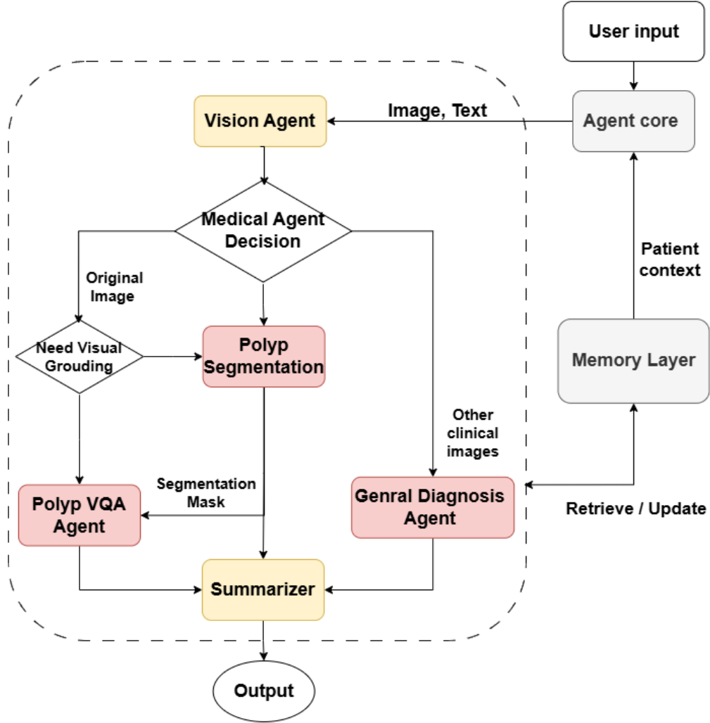
Figure 3.6: Vision Module workflow with routing, optional grounding, summarization, and memory context
