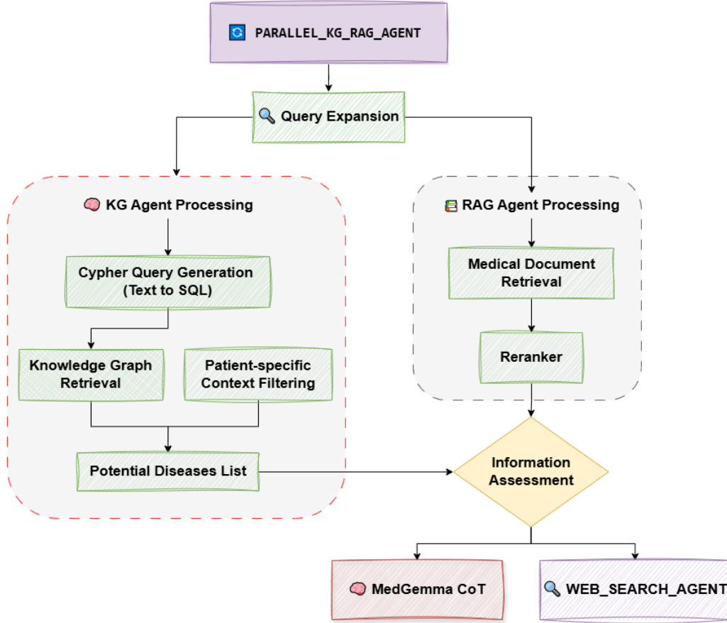
Figure 3.4: Parallel KG-RAG processing in the Text Module
